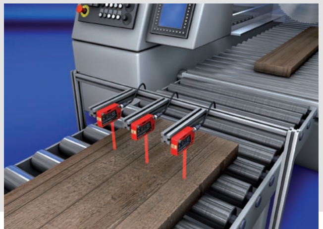
Detection of wood pallets
