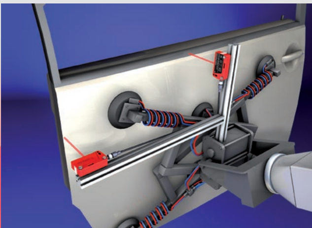
Positioning of a robotic arm
